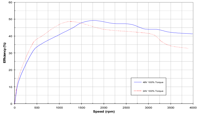
SilverMax 23H-1 Efficiency vs. Speed Data
