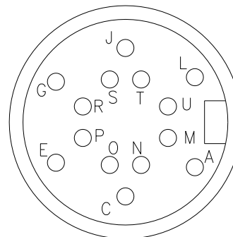
EXPOSED FRONT VIEW OF MOTOR CONNECTOR
